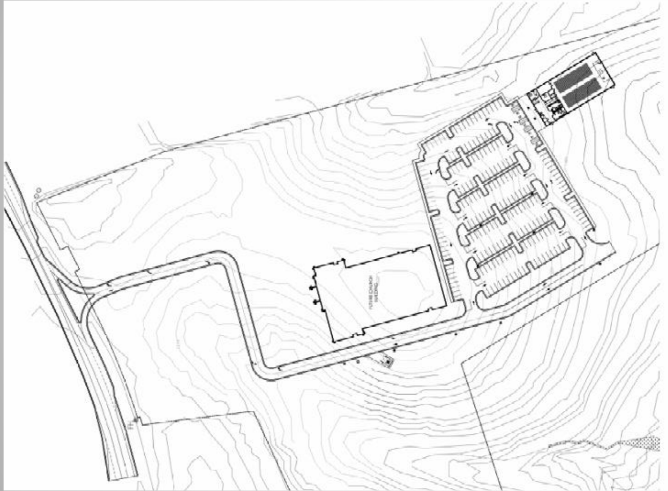
Site Plan
